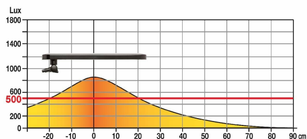
LUX measurement 40 cm above work surface
