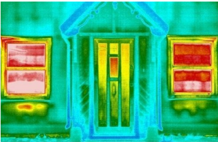
Both windows have radiators on the wall below them. The right-hand window's radiator is fitted with Radflek, which has reduced heat loss through the wall by 45%. This can be seen by the more muted colour below that window compared with below the left-hand window
