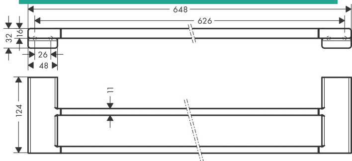
Concealed screw fitting
